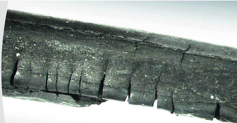
Extreme thermal stress on an O-ring
