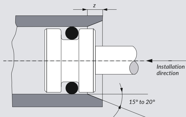
Installation angle for piston seals
