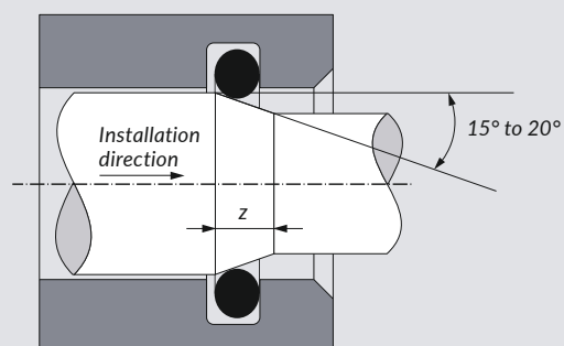
Installation angle for rod seals
